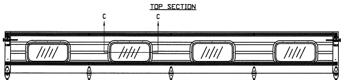
OPTIONAL GLAZED SECTION W/ 26' X 13' WINDOWS N.T.S.
