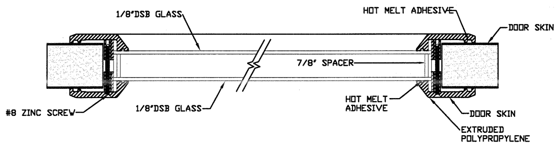
SECTION D-D 24' X 12' WINDOW DETAIL W/ 1-1/8\"/>
