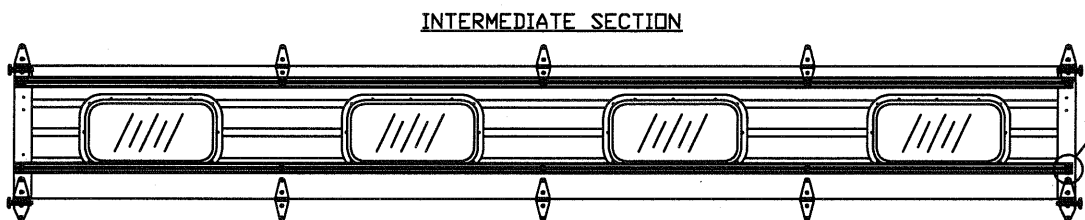
OPTIONAL GLAZED SECTION W/ 26' X 13' WINDOWS N.T.S.
